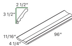
MOLDING CM6
