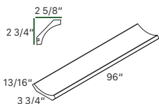
MOLDING CM4
